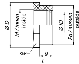
Dimensions Design A
