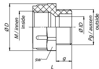
Dimensions Design B
